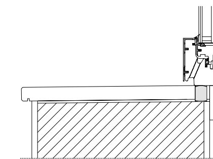
installation flush with the wall, removing old window, window lower section
