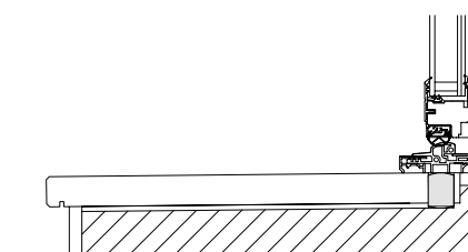
installation flush with the wall, keeping old window, window lower section
