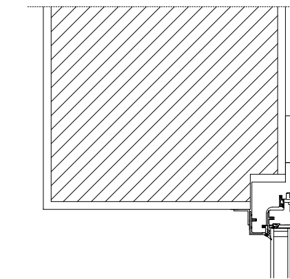
installation flush with the wall, removing old window, upper and lateral section
