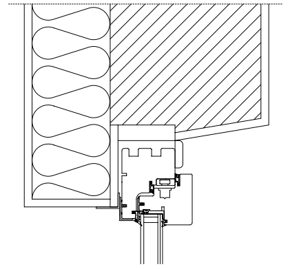
installation middle wall, upper and lateral section
