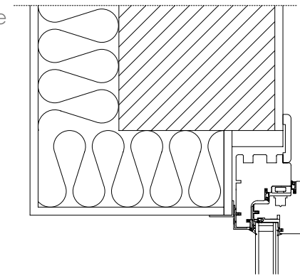
installation flush with the wall, upper and lateral section
